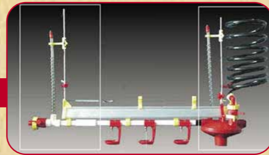
Nipple drinking line, with drip-catcher and anti-perching aluminium bar.
